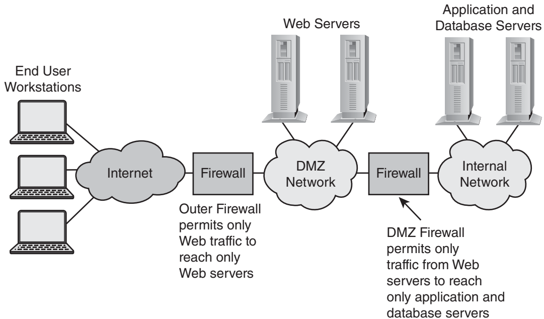
Figure 3-6 Typical DMZ network architecture protected by firewalls
