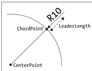
Figure 11-6. A radial dimension
